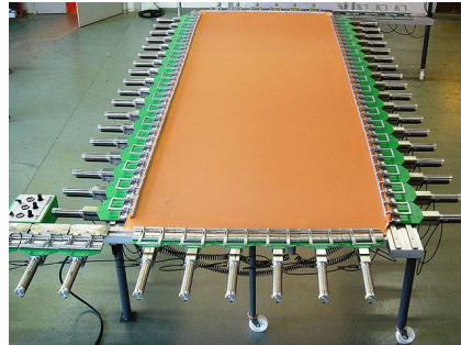
Large Format Screen Support
