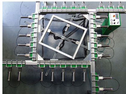
G-STRETCH 208P1 Pre-Bowing Device Installed
