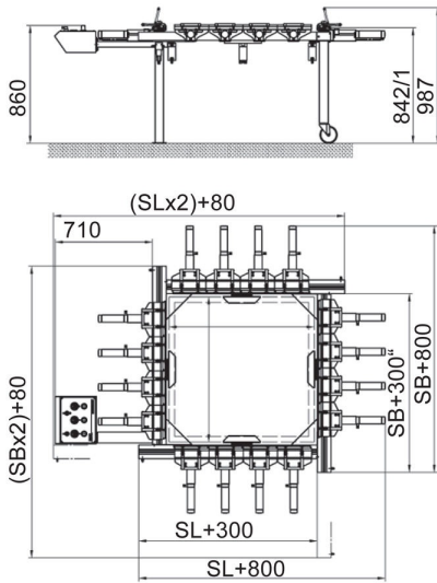
G-STRETCH 215 Dimensions (mm)
