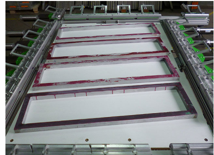
Optional Support Plate (Option Z)
