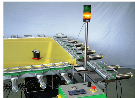
G-STRETCH 215A Variant Programmable Touchscreen Control Unit
