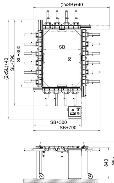
G-STRETCH 215A Dimensions (mm)
